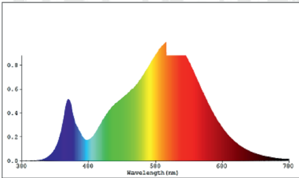
Model: LED Module of 88581-50 (3000K)
