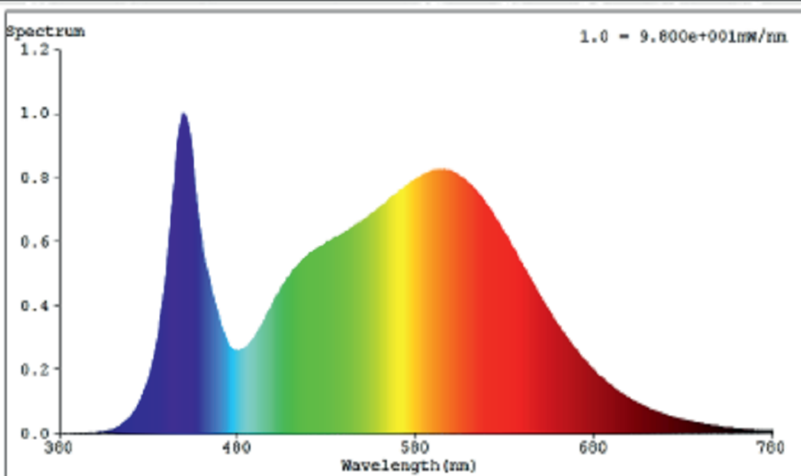
Model: LED Module of 88581-50 (6500K)
